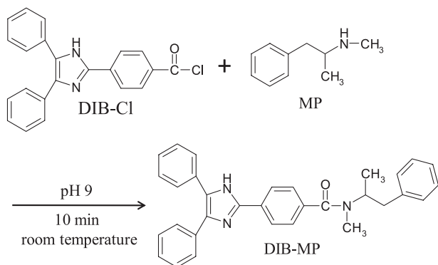
Fig. 3. Reaction Scheme of MP with DIB-Cl
