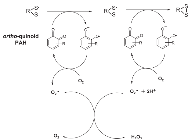
Fig. 3. Redox Cycle for Overproducing H_2O_2 by ortho -quinoid PAH
