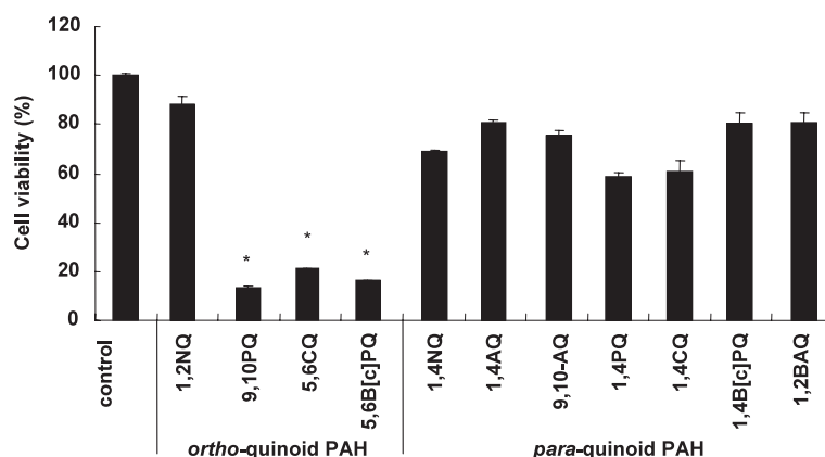
Fig. 1. Cellular Toxicity of Quinoid PAHs
