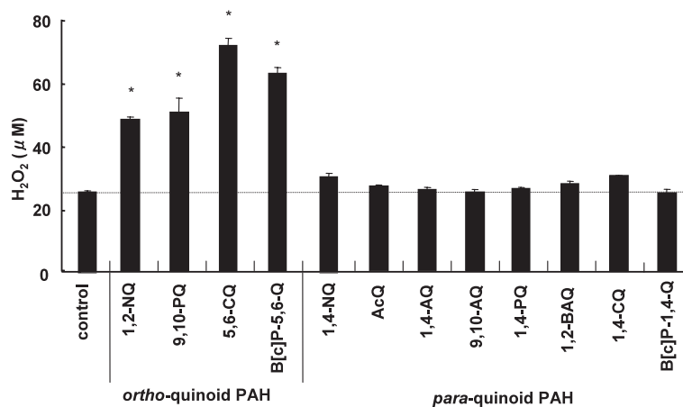
Fig. 2. Different Effect of ortho - and para -quinoid PAHs on H 2 O 2 Production in A549 Cells
